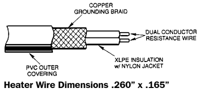
Figure 6 HEATER WIRE
